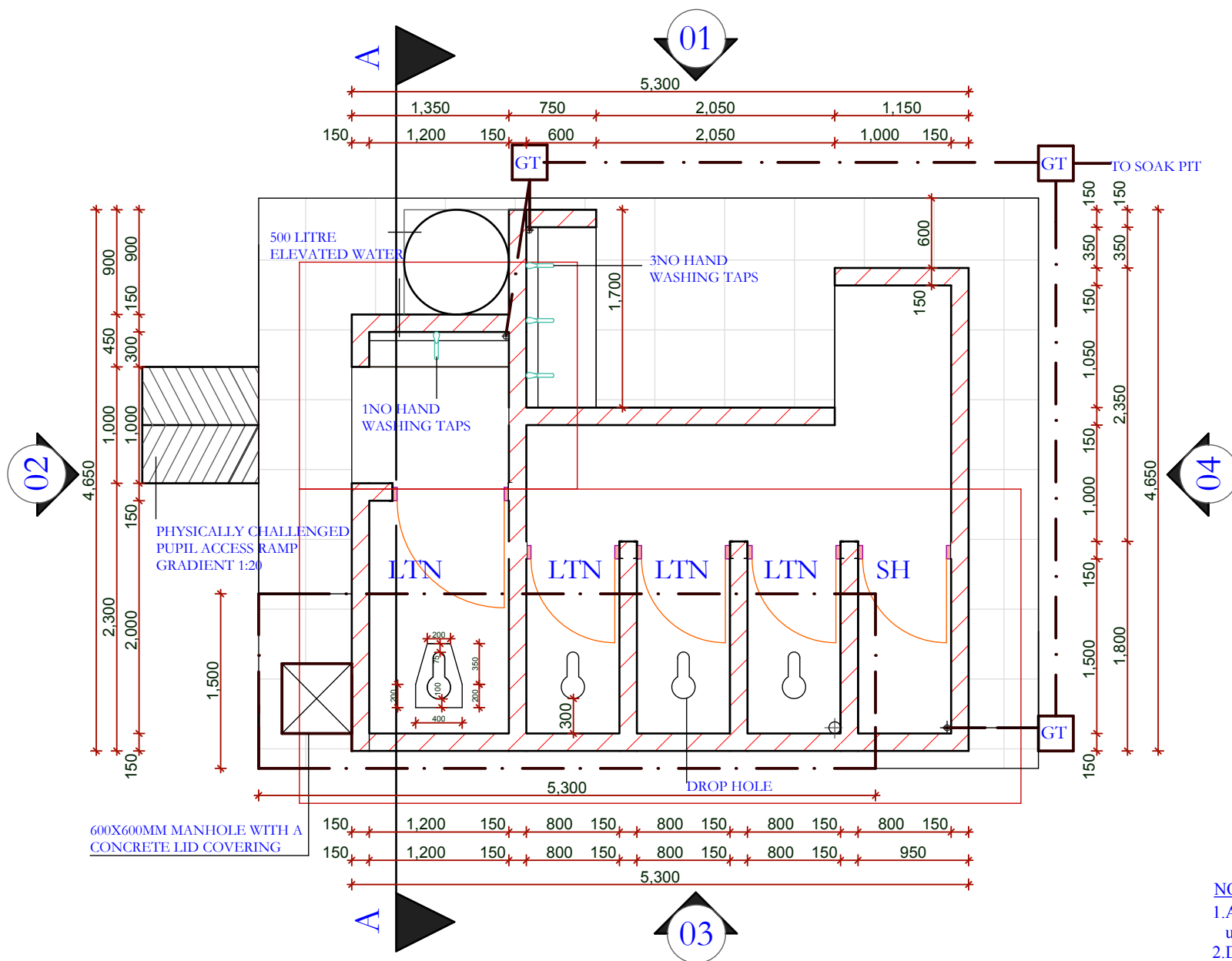
FLOOR PLAN GIRLS
